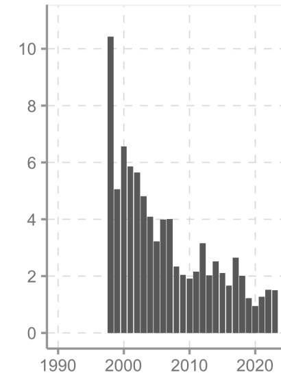
Endoftalmiter / 10 000 operationer
